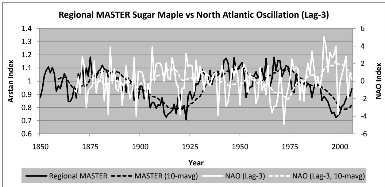
Figure 5.4. The standardized index of the regional master sugar maple tree-ring chronology plotted against the NAO at a three year lag. The curves of both the annual variability and smoothed decadal variability (10 year moving average) are plotted for visual comparison.
