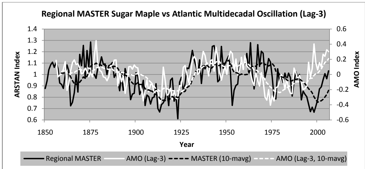
Figure 5.3. The standardized index of the regional master sugar maple tree-ring chronology plotted against the AMO at a three year lag. The curves of both the annual variability and smoothed decadal variability (10 year moving average) data are plotted for visual comparison.
