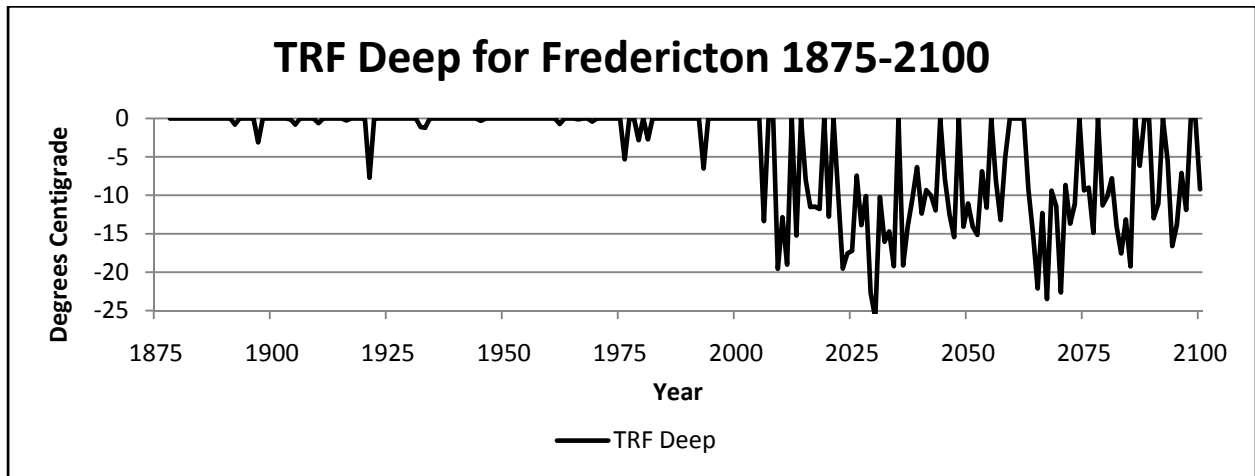
Figure 5.2. The Thaw/Refreeze Deep (TRF Deep) variable calculated using historical and forecast climate data for Fredericton is outlined. Noticeable is a large increase of occurrence in the data at the transition from historical to forecasted results around the year 2000.
