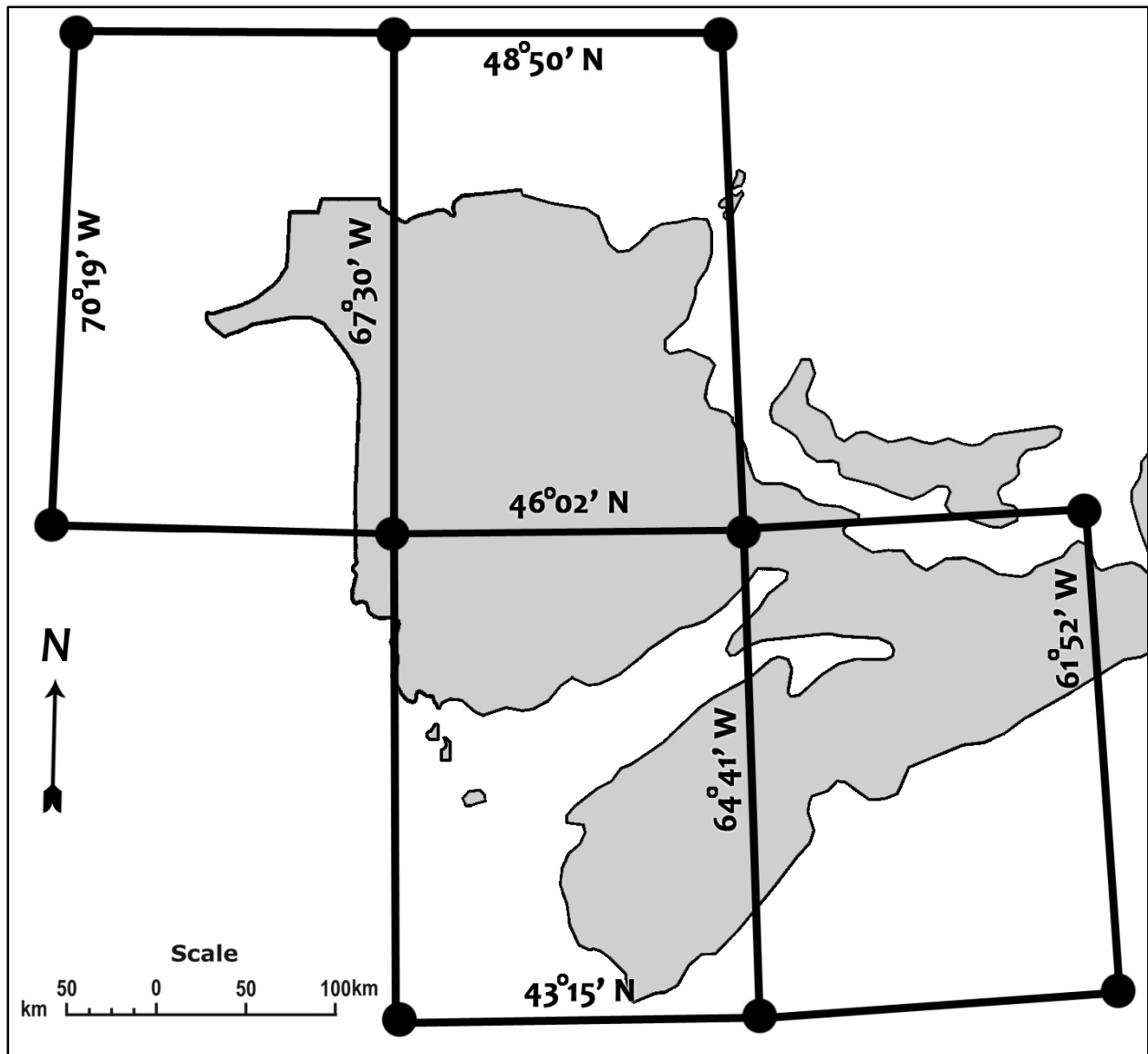
Figure 4.1. The CGCM3 produces a set of forecast data that is homogenous across a 2.81° X 2.81° grid square, and does so for a global grid. The CGCM3 output grid squares used in the study are illustrated over the Maritime provinces. Latitudinal and longitudinal boundaries for each grid square are also given. Base map © 2002. Her Majesty the Queen in Right of Canada, Natural Resources Canada.
